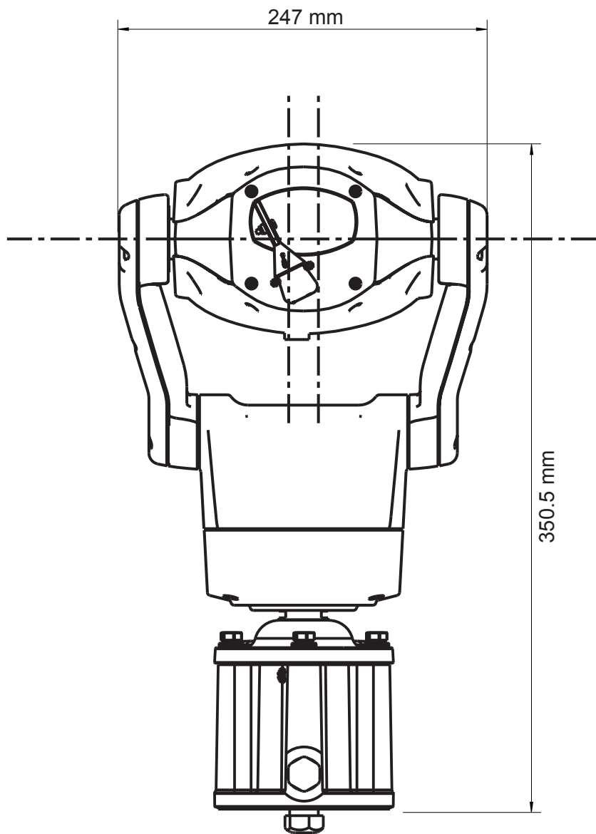
Vista frontal
