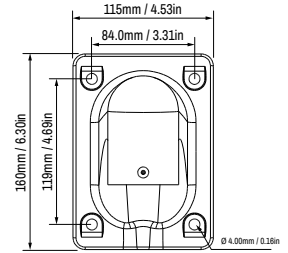
Wall Mount Bracket (Front Face)
